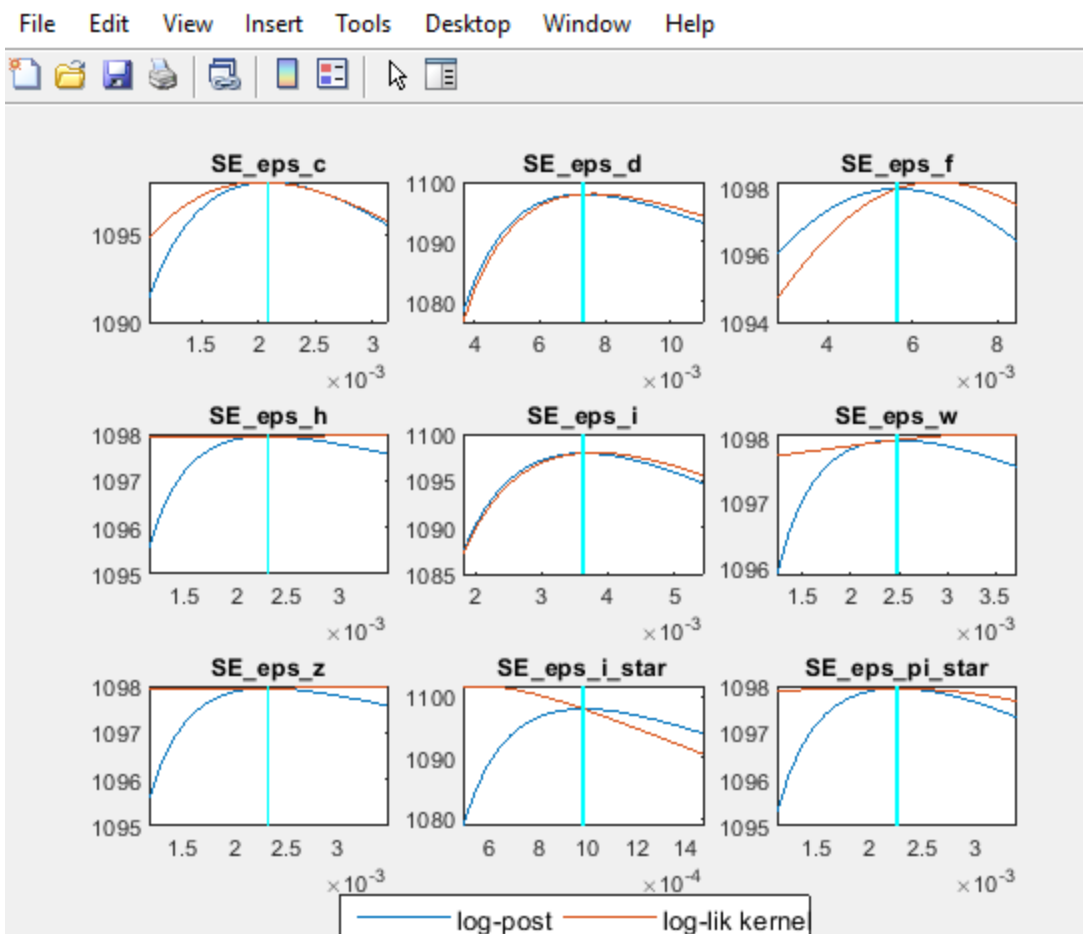
Figure 6: Mode check plots
