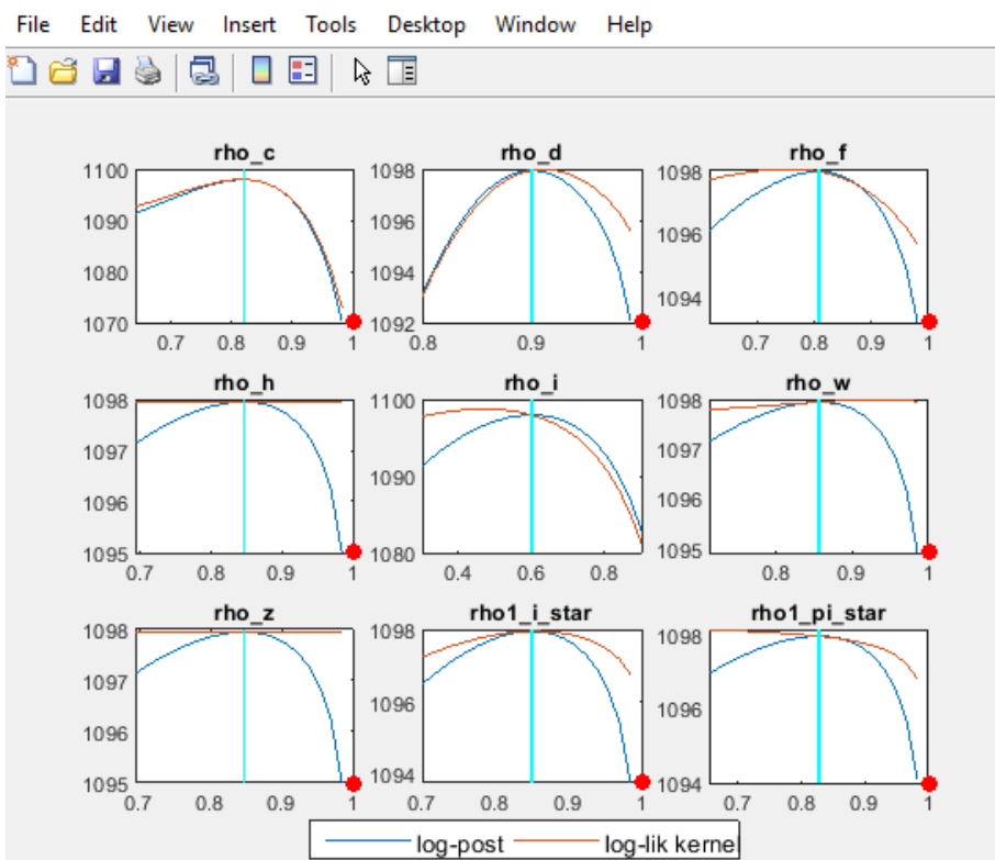
Figure 6: Mode check plots
