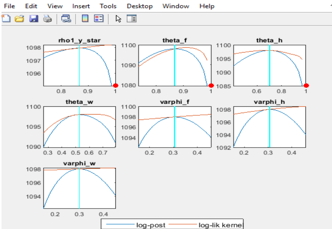
Figure 10: Mode check plots
