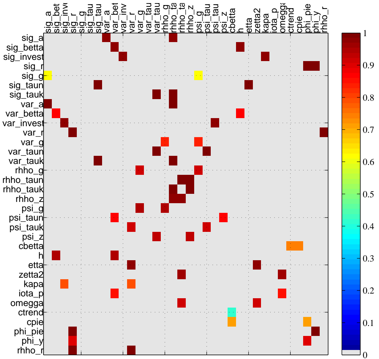
prior_mean – Collinearity patterns with 2 parameter(s)
