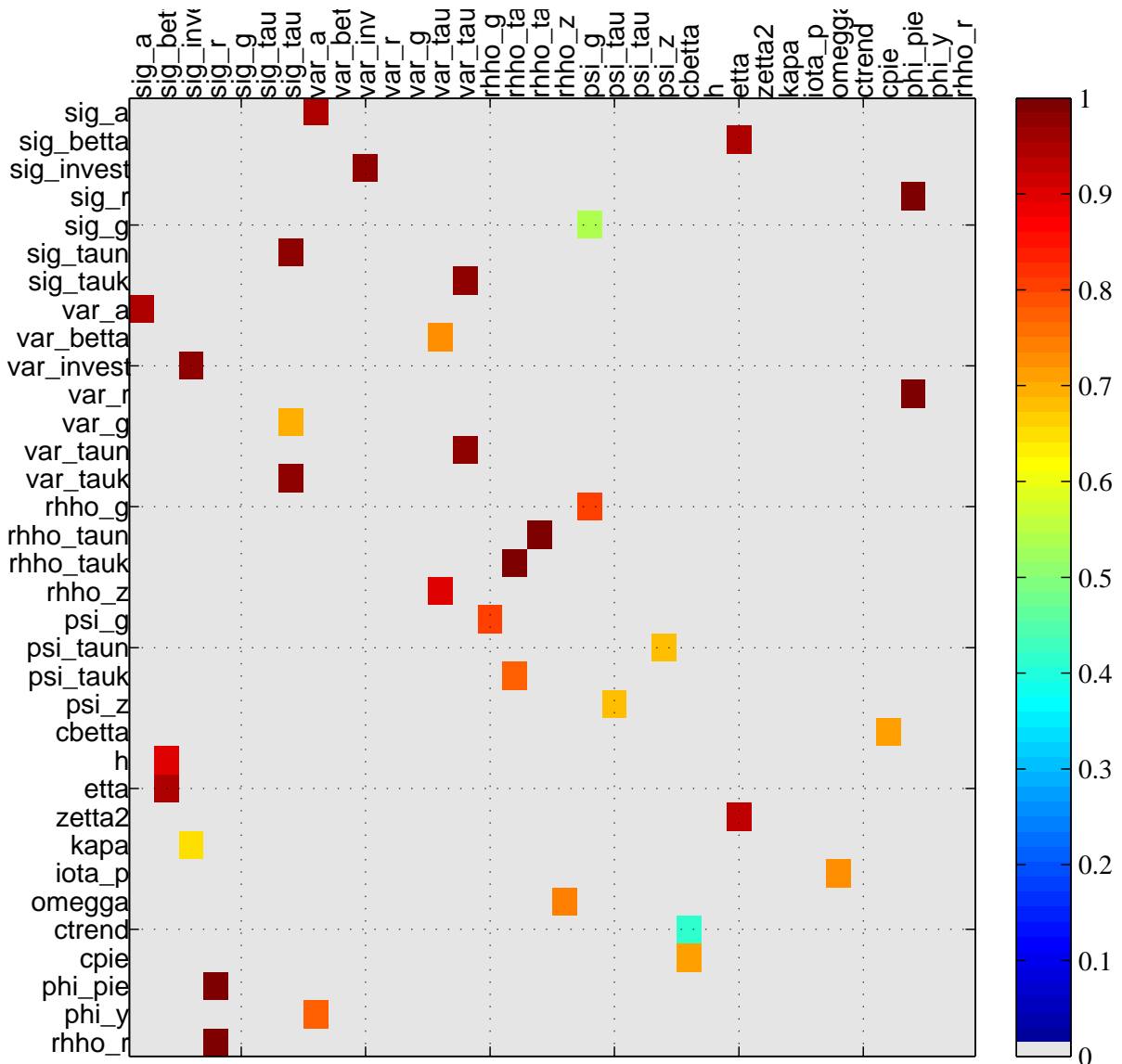
prior_mean – Collinearity patterns with 1 parameter(s)
