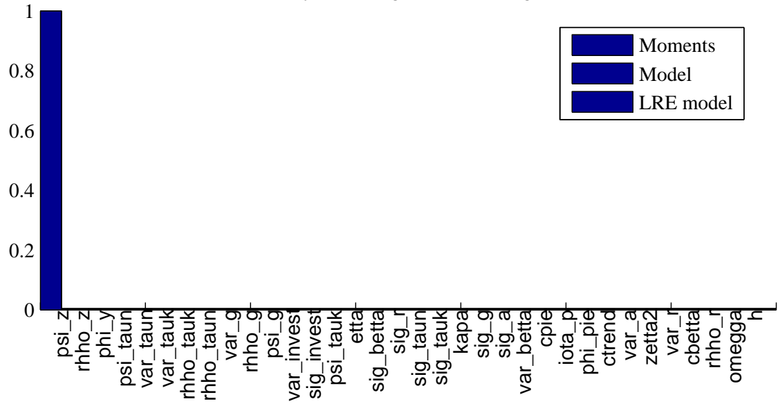
Sensitivity bars using derivatives (log-scale)
