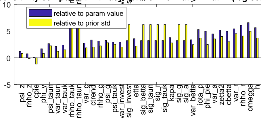
Sensitivity component with asymptotic Information matrix (log-scale)
